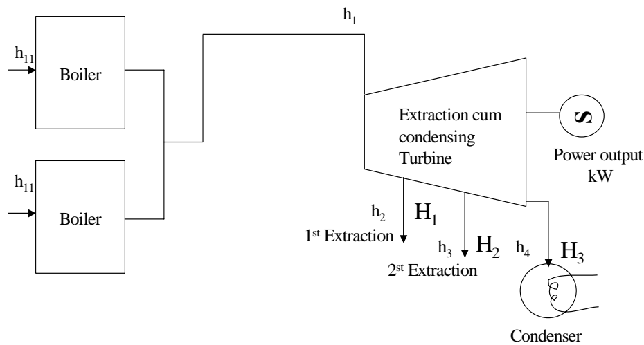
Figure 3.1 Process Flow Diagram for Cogeneration Plant
