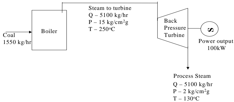
Figure 3.2 Process Flow Diagram for Small Cogeneration Plant
